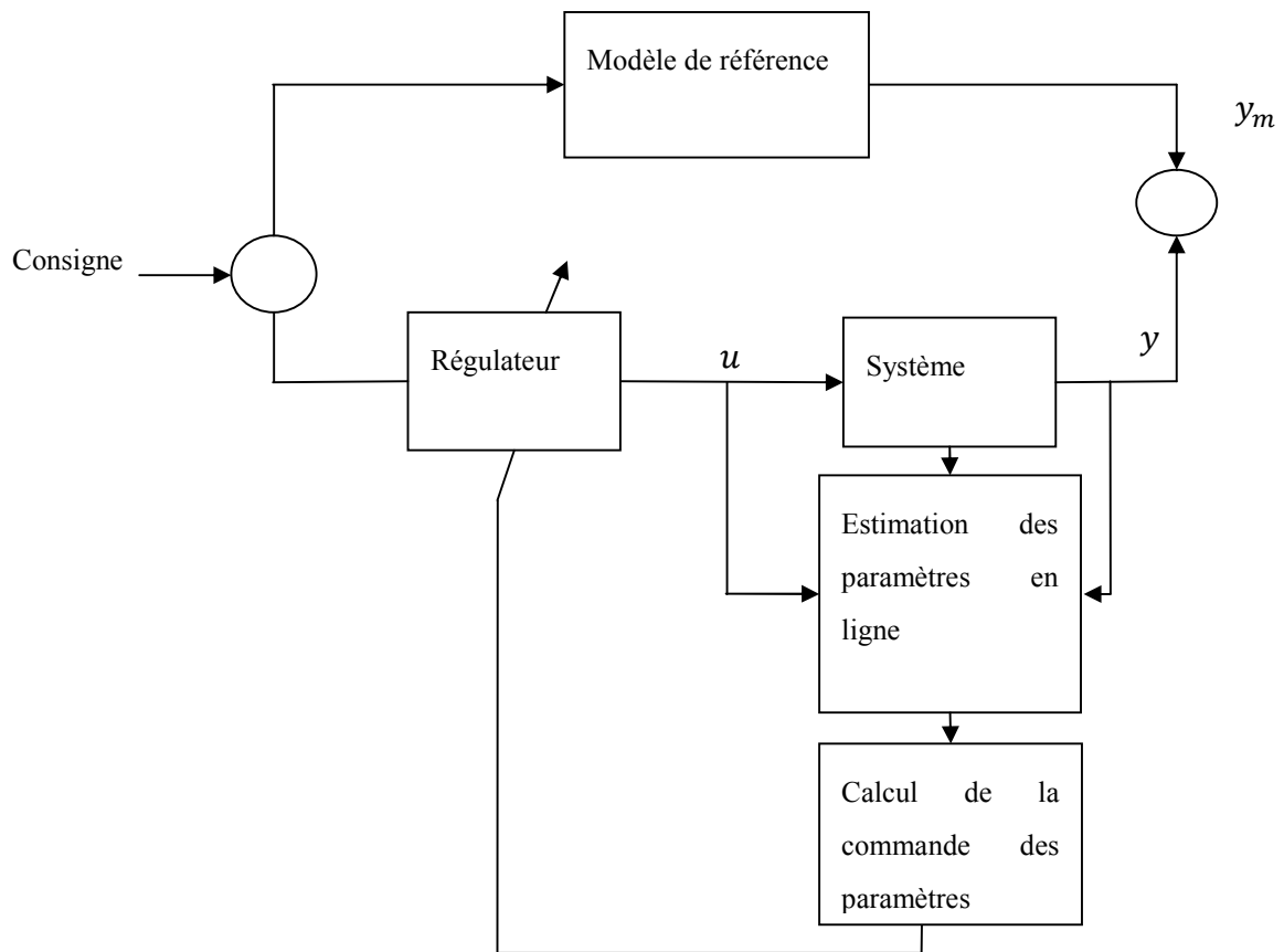
Figure II.8 : MRAC indirect.
