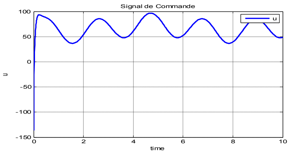
Figure III.7 : Signal de commande.
