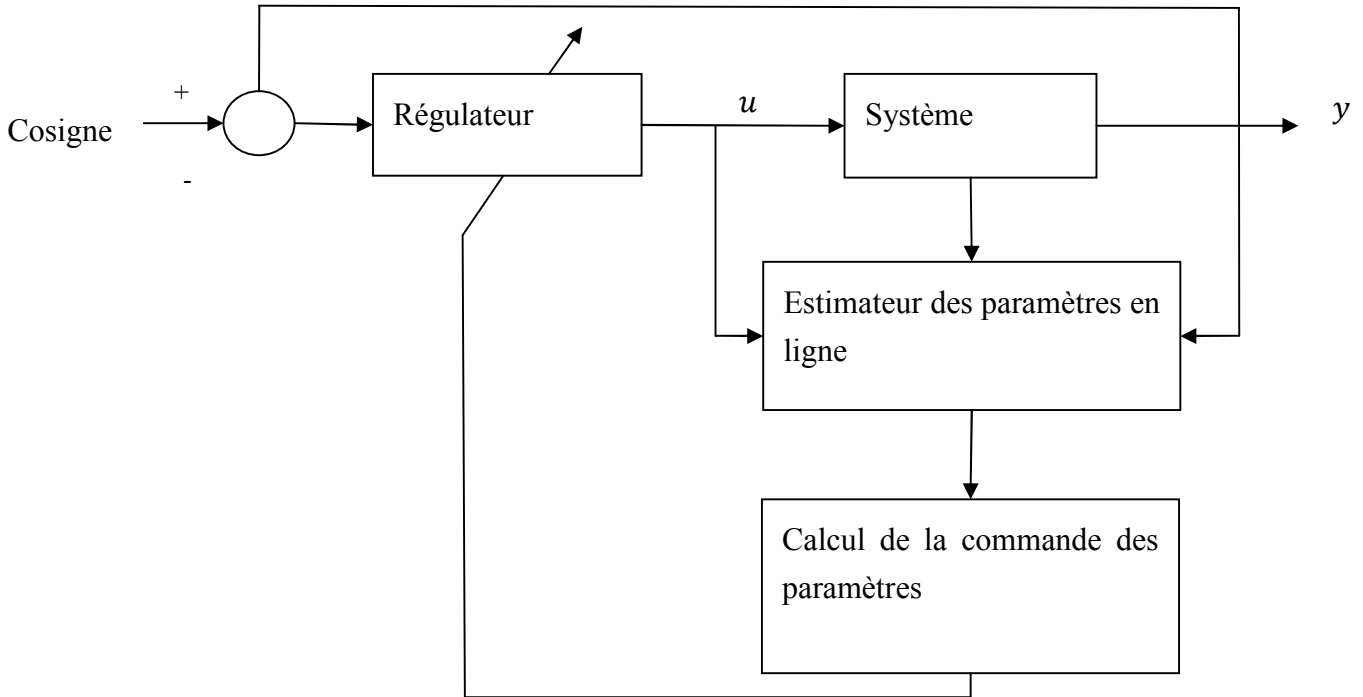
Figure II.3 : Commande adaptative indirecte.
